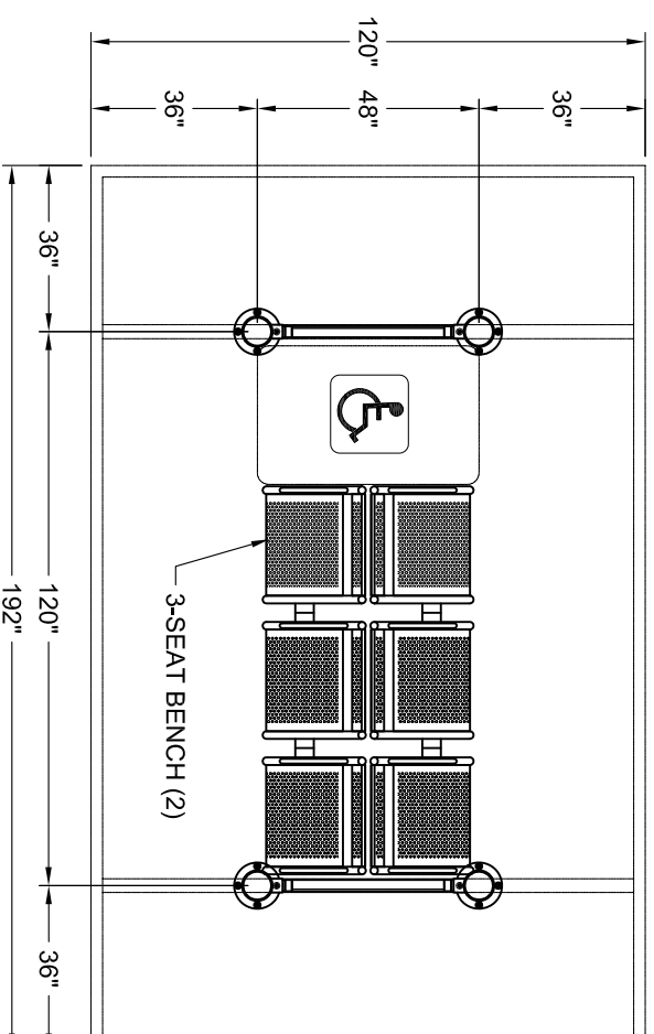
TYPE 2 ALTERNATE FLOOR PLAN NORTHBOUND STOP #1111
