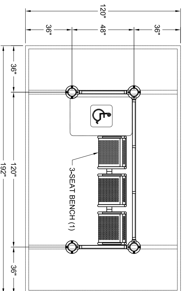
TYPE 2 STANDARD FLOOR PLAN EASTBOUND STOP #1093 WESTBOUND STOP #1094
